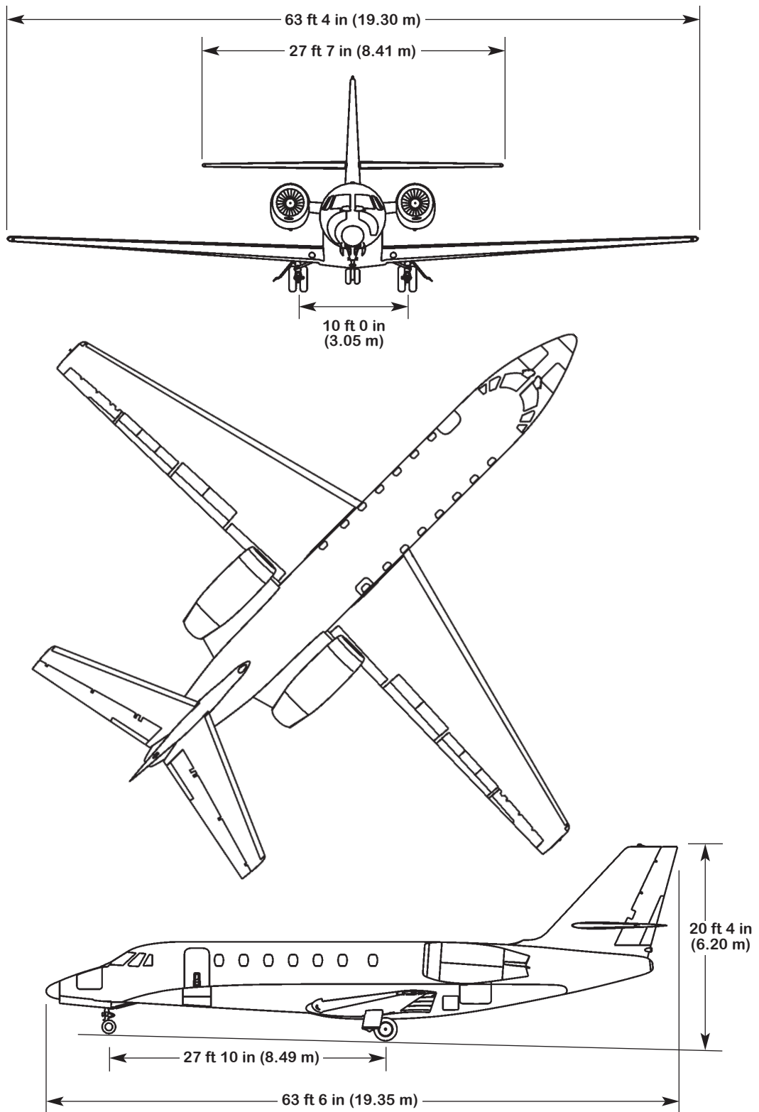
FIGURE I — CITATION SOVEREIGN EXTERIOR DIMENSIONS
