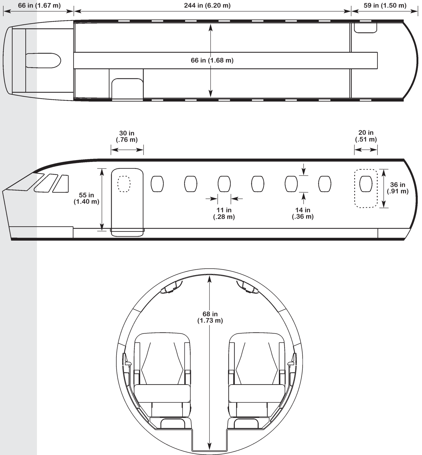
FIGURE II — CITATION SOVEREIGN INTERIOR DIMENSIONS
